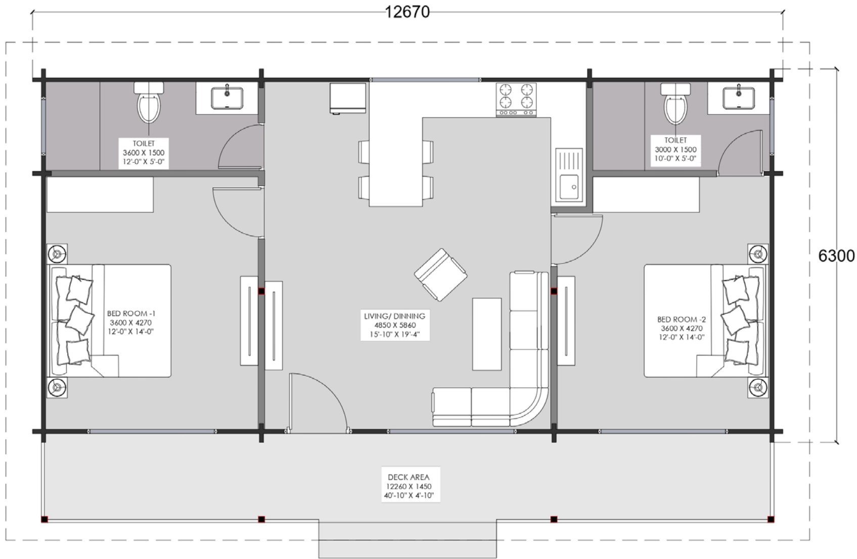
GROUND FLOOR PLAN AREA – 1000 SQ. FT.
